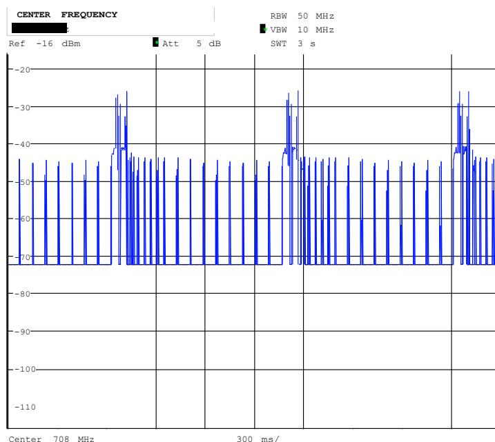
Figure B.3: Zero span plot of "short_UE-Video-Stream_V2" waveform (1 second loop)
