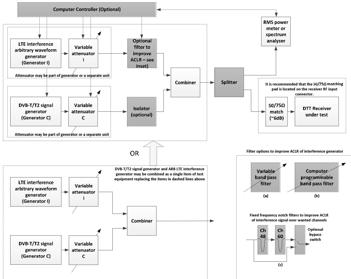
Figure 2: Generic measurement arrangement for adjacent channel selectivity, blocking and overloading tests
