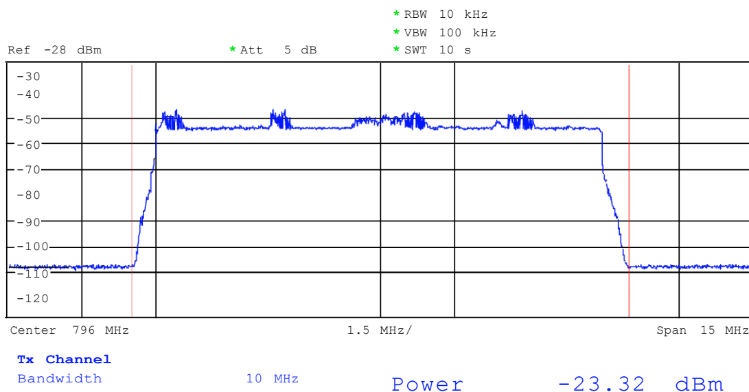
Figure B.5: Swept frequency plot of "LTE_BS-idle_V3_synth" waveform
