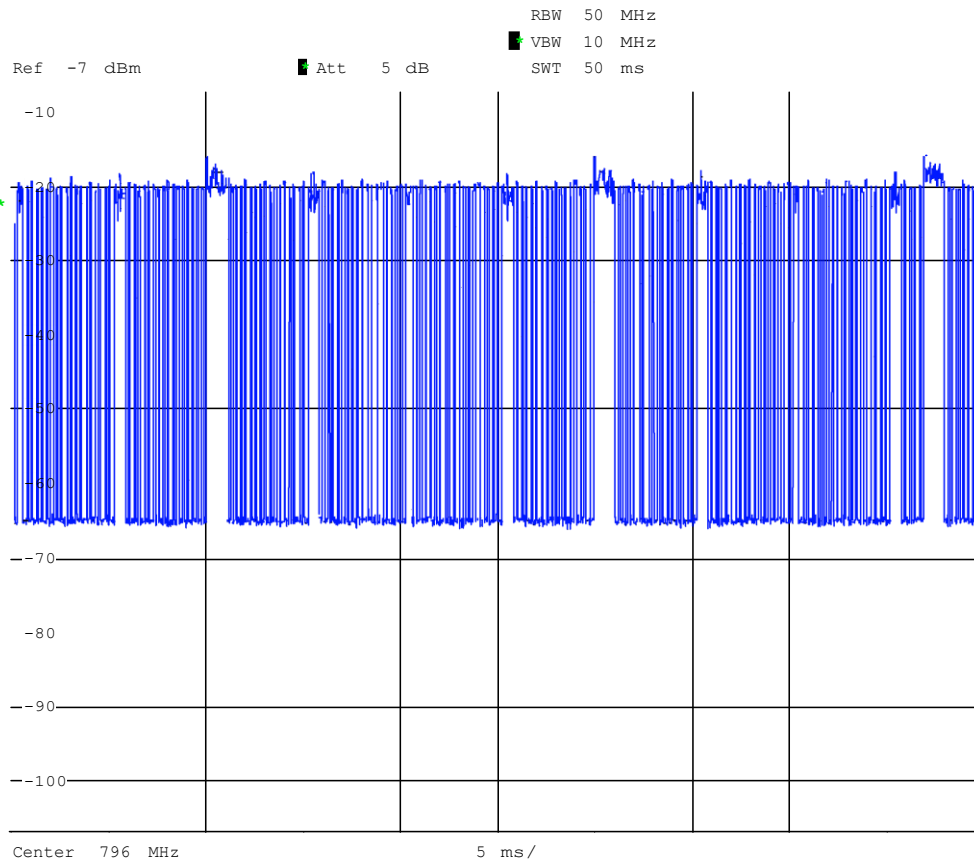
Figure B.4: Zero span plot of a 50 ms section of "LTE_BS-idle_V3_synth" waveform
