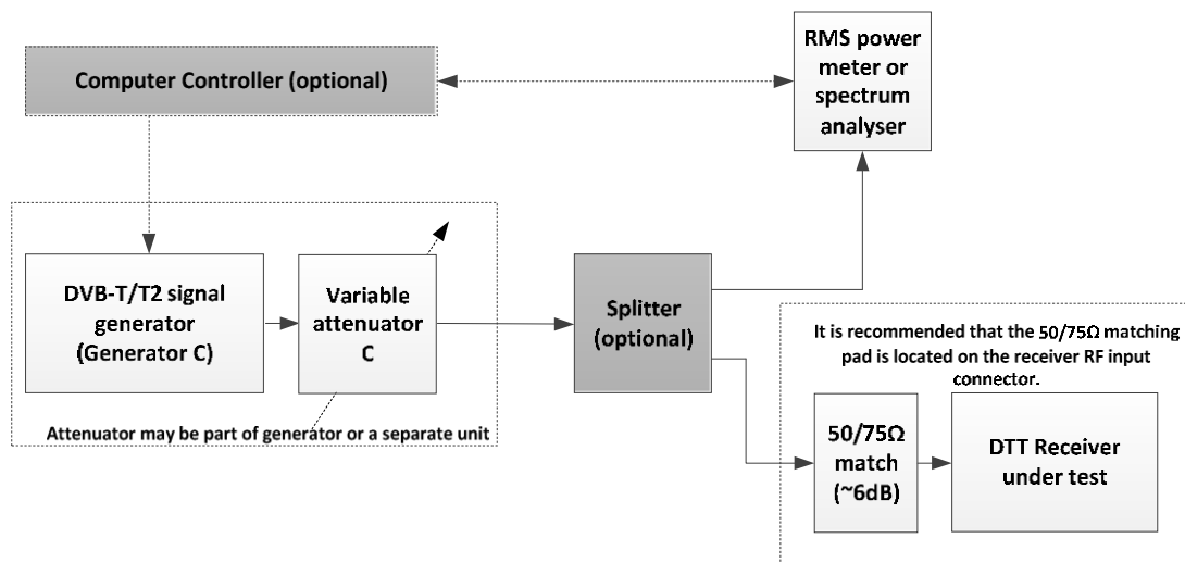
Figure 1: Measurement arrangement for sensitivity tests
