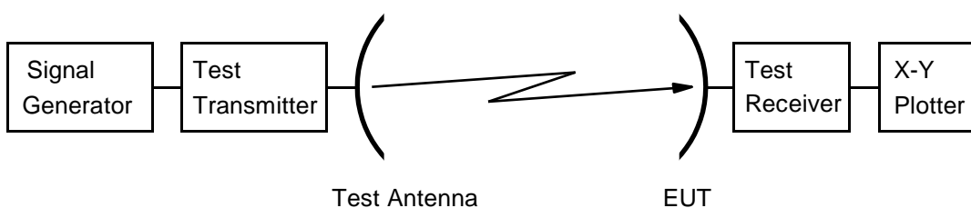
Figure 3: Test arrangement - antenna receive pattern measurement
